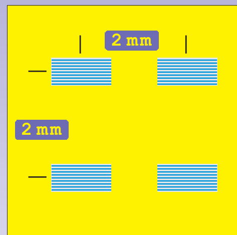
Layout of the standard nanograting template
